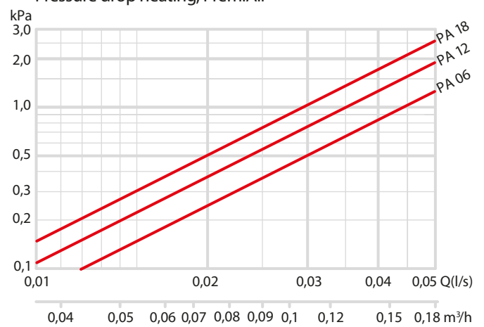
Diagram 6. Pressure drop heating, PremiAir
