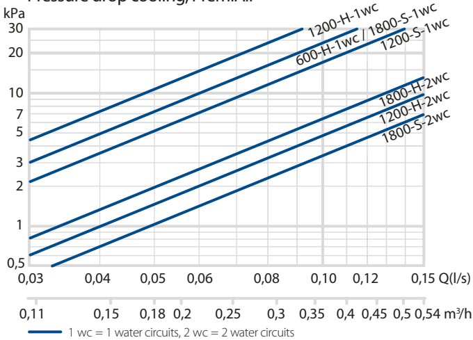
Diagram 5. Pressure drop cooling, PremiAir
