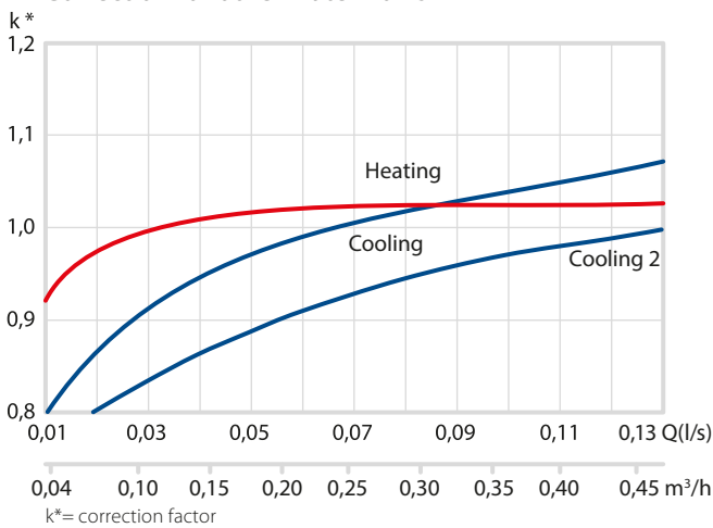
Diagram 4. Correction for other water flows
